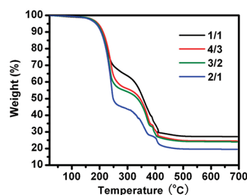
Figure 8. TGA curves of PSA@Fe 3 O 4 @SiO 2 -DMH nanoparticles prepared with different DMH/PSA@Fe 3 O 4 @SiO 2 -CPS mass ratio.
