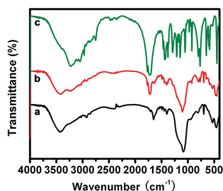
Figure 7. FTIR spectra of (a) PSA@Fe 3 O 4 @SiO 2 , (b) PSA@Fe 3 O 4 @SiO 2 -DMH nanoparticles, and (c) free DMH.
