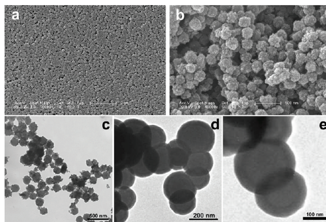
Figure 2. SEM images of (a) PSA and (b) PSA@Fe 3 O 4 , and (c) TEM images of PSA@Fe 3 O 4 , (d) PSA@Fe 3 O 4 @SiO 2 , and (e) N -halamine-immobilized PSA@Fe 3 O 4 @SiO 2 nanoparticles.
