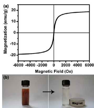
Figure 10. (a) Magnetization curve of the N -halamine-immobilized PSA@Fe 3 O 4 @SiO 2 nanoparticles at 298 K. (b) Photographs of the N -halamine-immobilized PSA@Fe 3 O 4 @SiO 2 nanoparticles dispersed in aqueous solution without and with external magnetic field.
